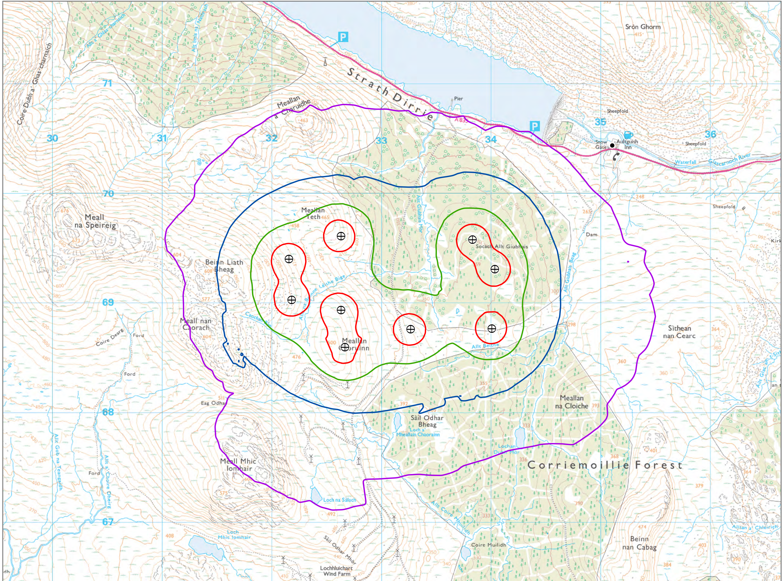
Figure 8.2: Noise Contour Plot
